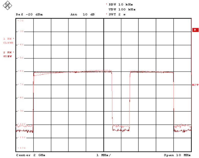
Fig. 24 FSP Demo Trace
