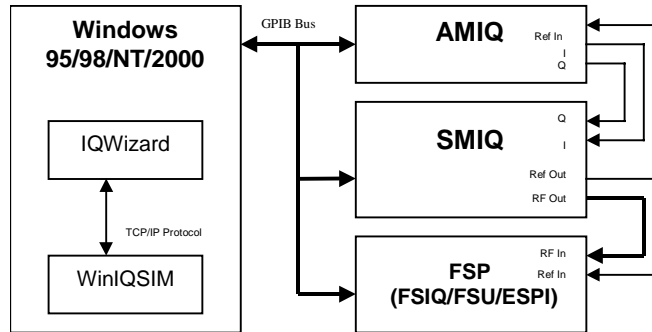
Fig. 16 Demo Hardware Configuration
