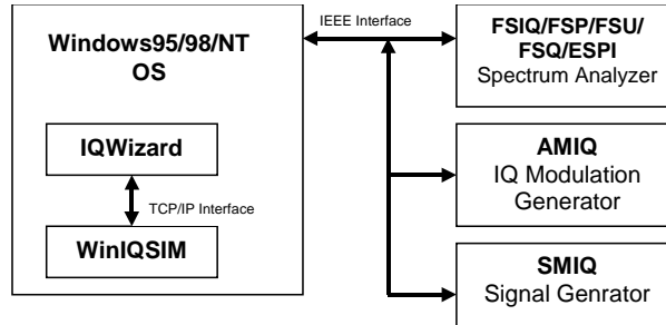
Fig. 1 Connecting Instruments
