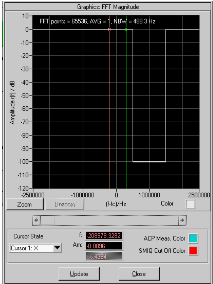
Fig. 20 WinIQSIM Orig. Signal
